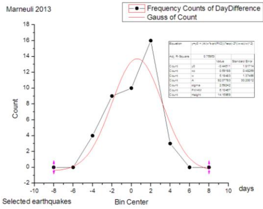
Fig.5 Marneuli borehole Gauss Distribution for day difference (2013)
