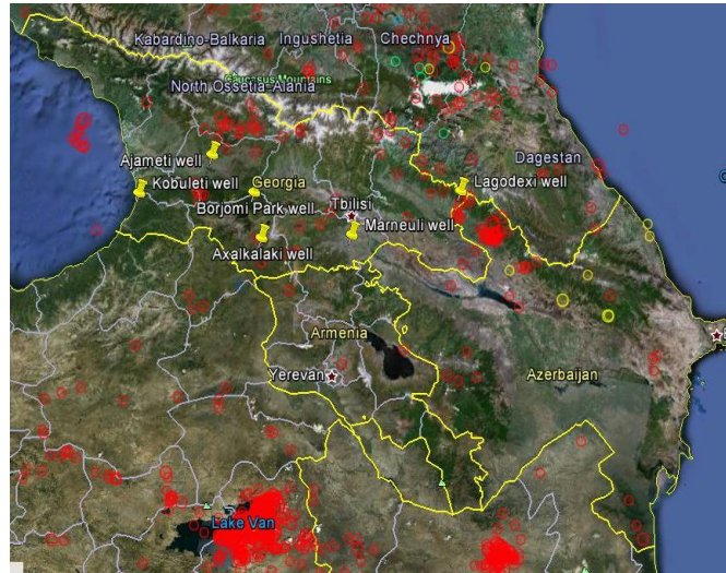
Fig.1b The map of earthquakes during 2011-2012
