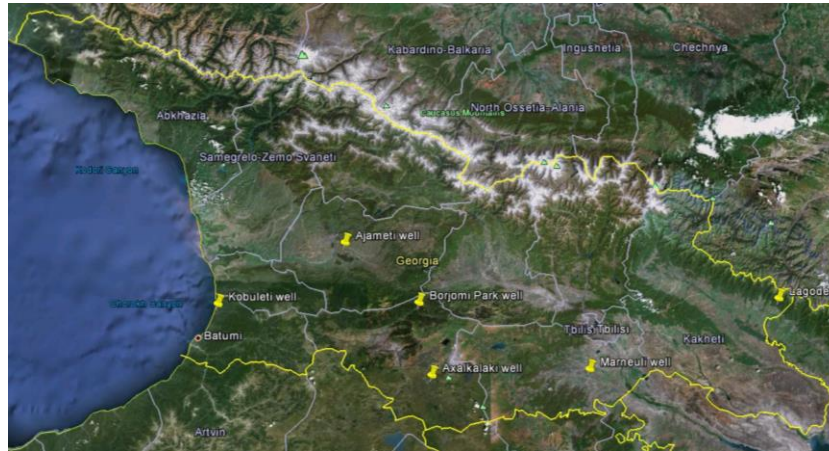
Fig. 1a Map of boreholes in Georgia
